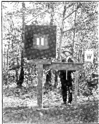
Fig. 2 —Background and Test Object used in determining effect of Stereoscopic Vision on discrimination of detail
